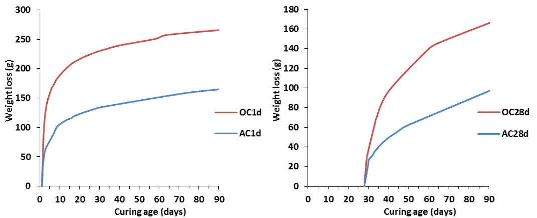
Figure 1: Weight loss of AC and OC exposed at 1 day (left) and 28 days (right)
