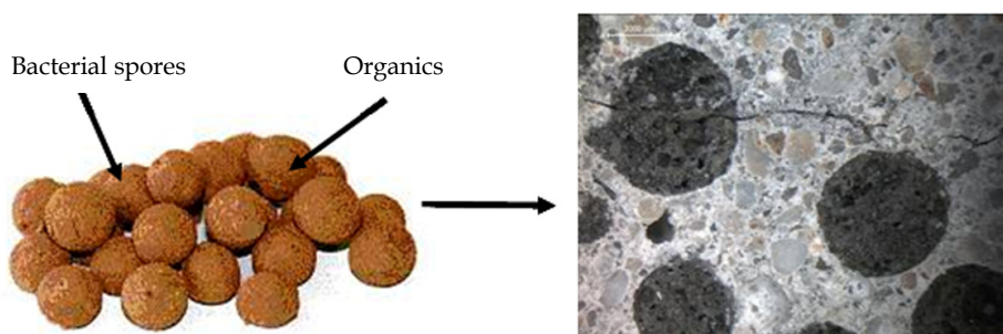
Figure 2. Self healing admixture composed of expanded clay particles (left) loaded with bacterial spores and organic bio-mineral precursor compound (calcium lactate). When embedded in the concrete matrix (right) the loaded expanded clay particles represent internal reservoirs containing the two-component healing agent consisting of bacterial spores and a suitable bio-mineral precursor compound.
